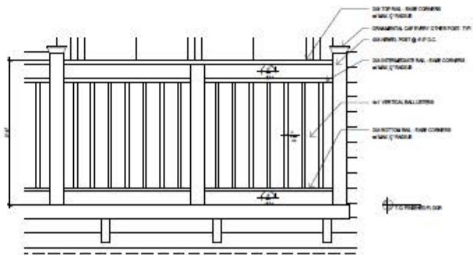
EXTERIOR GUARDRAIL @ WALL DETAIL 1/4" = 1'-0" 1
